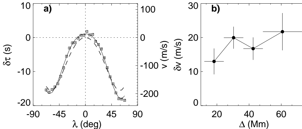
Figure 2. (a) Reciprocal travel-time differences for east-west propagating waves, as a function of latitude, and the inferred flow velocity (see text). The solid curve is a fit to the observations, and the dashed curve is the measured surface rotation rate. Note that the solid-body component of the equatorial surface rate has been subtracted from all the velocities. (b) Inferred velocity difference between northern and southern hemispheres, as a function of wave travel distance. The velocities were taken at \pm 60^\circ latitude. The sense of the asymmetry is that the southern hemisphere is rotating more rapidly.
