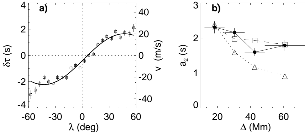
Figure 1. (a) Reciprocal travel-time differences for north-south propagating waves, as a function of latitude, and the inferred flow velocity (see text). (b) Observed travel-time differences as a function of distance travelled. The observed values are shown as the filled circles, with errors. The horizontal error bars indicate the range of distances included in the measurement for each point. Also shown are the calculated coefficients for two different flow models, both of which vary with latitude according to v = v_0 \sin 2\lambda . In one model (open squares) the velocity is constant with depth and the magnitude v_0 = 23.5 m/s. In the second (open triangles), the flow is constant to a depth of 9.3 Mm and zero in the deeper layers.
